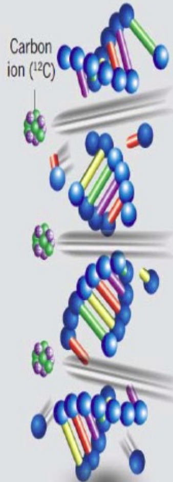
Carbon-ion beam
